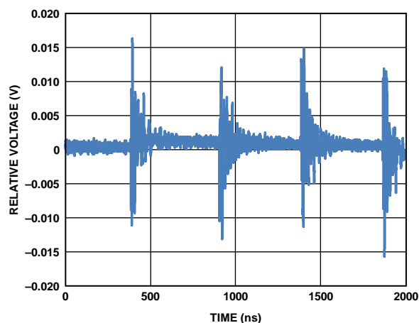
Figure 28. Digital Feedthrough
