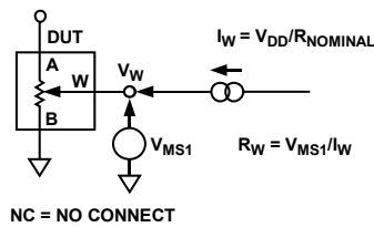
Figure 33. Wiper Resistance
