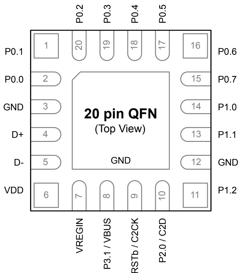
Figure 6.3. EFM8UB1x-QFN20 Pinout
