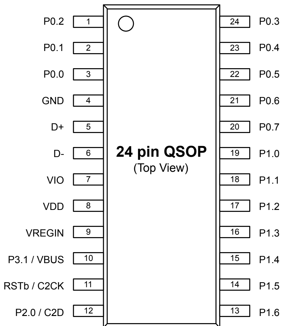
Figure 6.2. EFM8UB1x-QSOP24 Pinout
