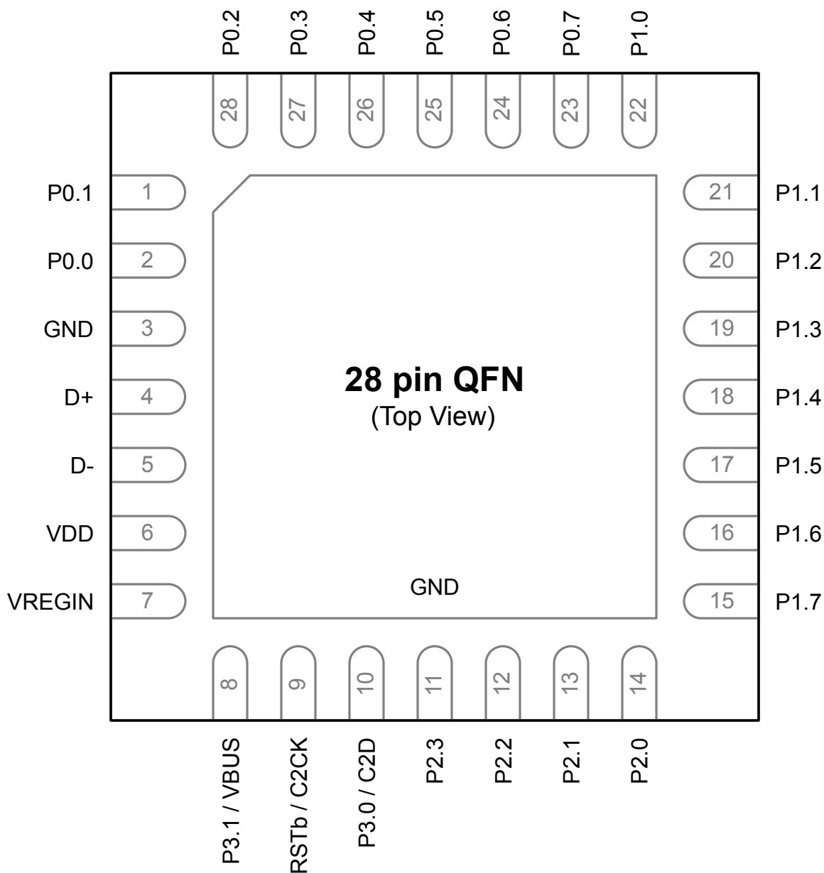
Figure 6.1. EFM8UB1x-QFN28 Pinout
