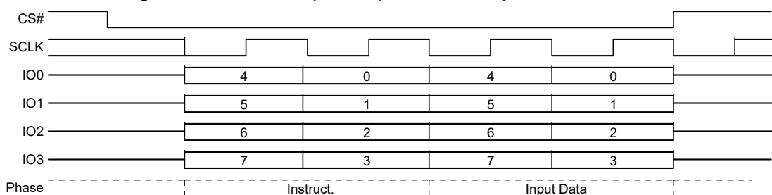
Figure 52. Write DLRV (WDLRV) Command Sequence – QPI Mode
