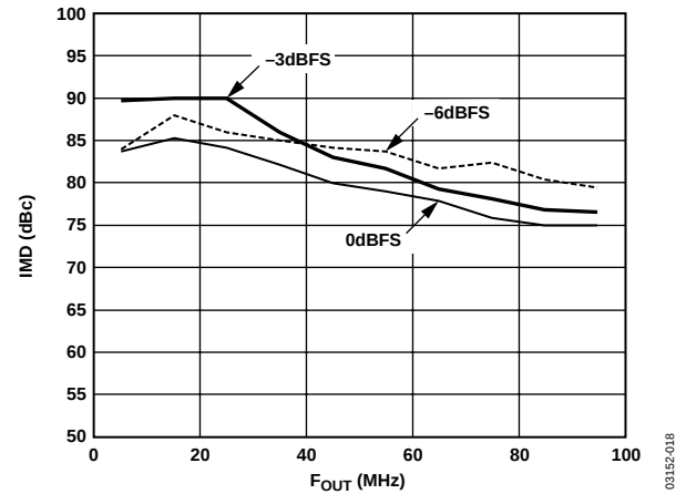
Figure 18. Third-Order IMD vs. Frequency, f_{DATA} = 200 MSPS, 1x Interpolation
