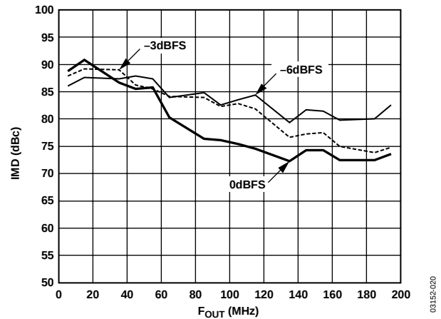
Figure 20. Third-Order IMD vs. Frequency, f_{DATA} = 50 MSPS, 8x Interpolation
