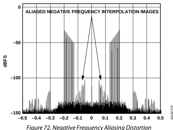
Figure 72. Negative Frequency Aliasing Distortion
