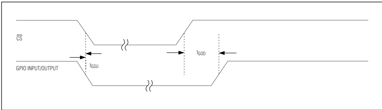
Figure 13. GPIO Timing
