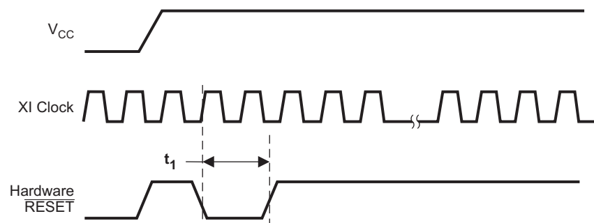
Figure 9-2. Reset Timing
