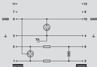
Complete module, floating ground
