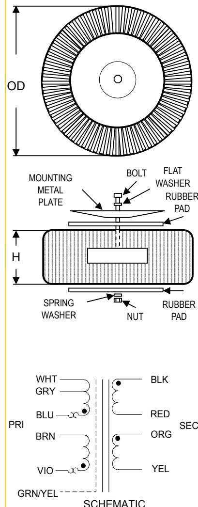
SCHEMATIC
