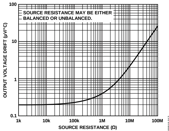
Figure 12. Offset Voltage Drift vs. Source Resistance
