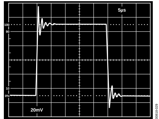
Figure 29. Unity Gain Follower Small Signal Pulse Response R_F = 0\text{ }\Omega , C_L = 1000\text{ pF}
