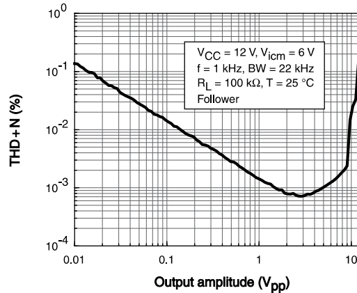
Figure 21: Distortion and noise vs. amplitude at V_{ictm} = V_{CC}/2 and V_{CC} = 12\text{ V}
