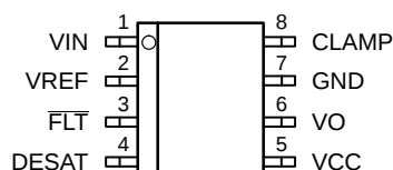
NCV5701A
