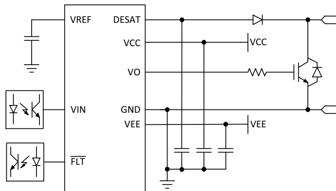
NCV5701B
