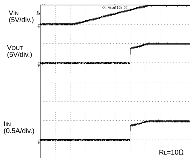
TIME(10ms/div.) Figure 40. UVLO Response Increasing V_{IN}
