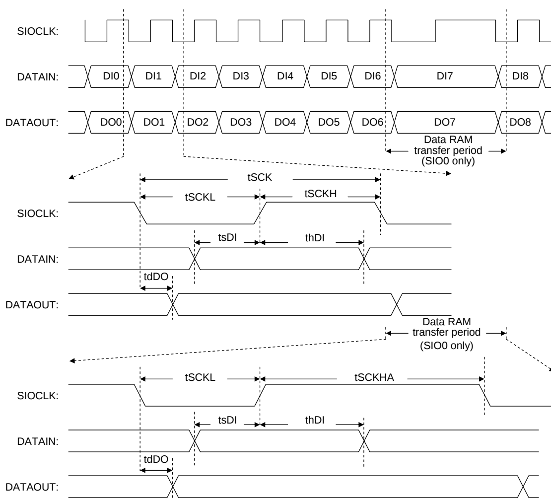
Figure 6 Serial I/O Waveforms
