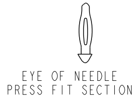
DETAIL A SCALE 4:1 SEE NOTE 16
