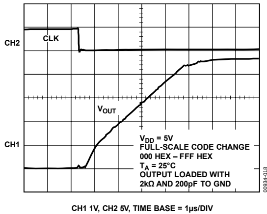
Figure 18. Full-Scale Settling Time
