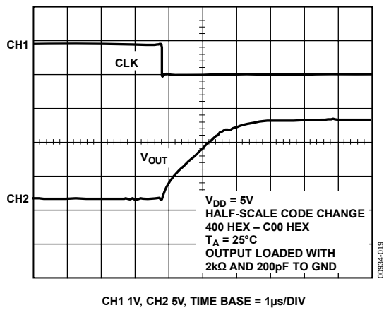
Figure 19. Half-Scale Settling Time
