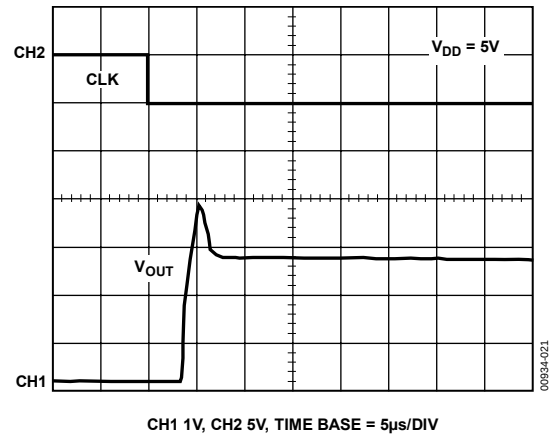
Figure 21. Exiting Power-Down (800 Hex Loaded)
