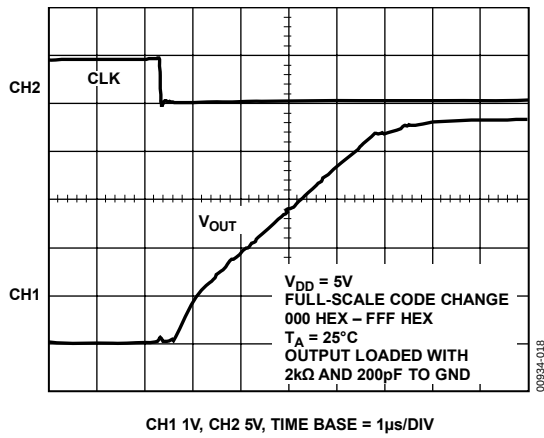
Figure 18. Full-Scale Settling Time
