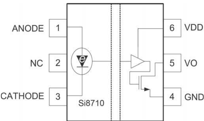
Figure 14. Pin Configuration
