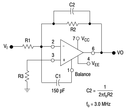
Figure 15. Feedforward Compensation
