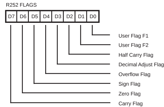
Figure 57. Flag Register FCH: Read/Write
