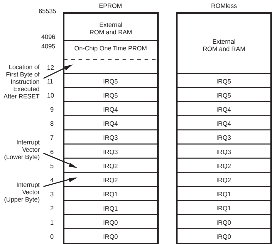
Figure 22. Program Memory Map (ROMless Z86E40 Only)
