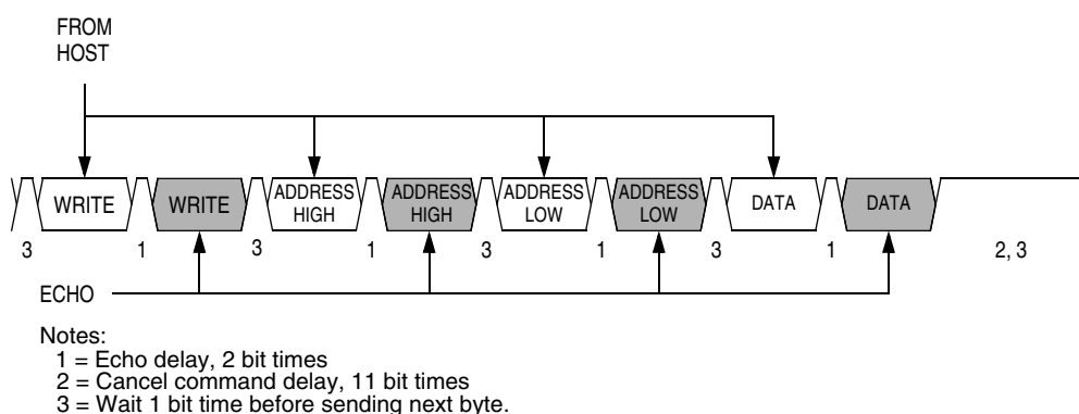
Figure 15-6. Write Transaction
