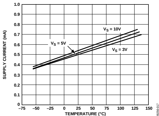
Figure 12. Supply Current/Amplifier vs. Temperature
