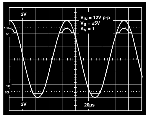
Figure 25. No Phase Reversal ( V_{IN} = 12\text{V p-p} , V_S = \pm 5\text{V} , A_V = 1 )
