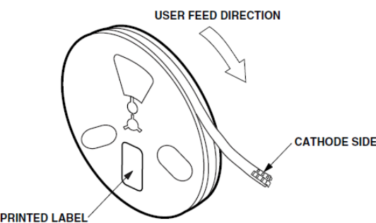
Figure 12: Reel Orientation
