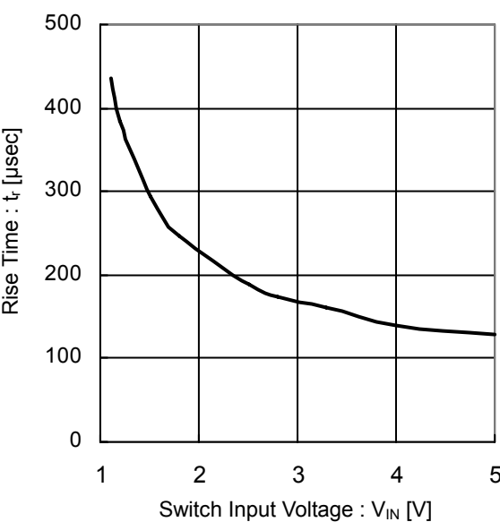
Figure 45. Rise Time vs Switch Input Voltage (BUS1DJC3GWZ)
