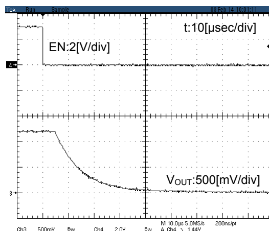
Figure 33. Turn OFF Response 1 (BUS1DJC0GWZ V_{IN}=1.2V )
