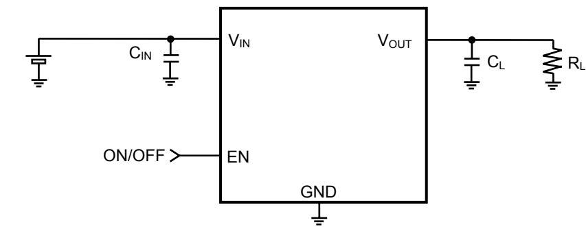
Figure 4. Measurement Circuit
