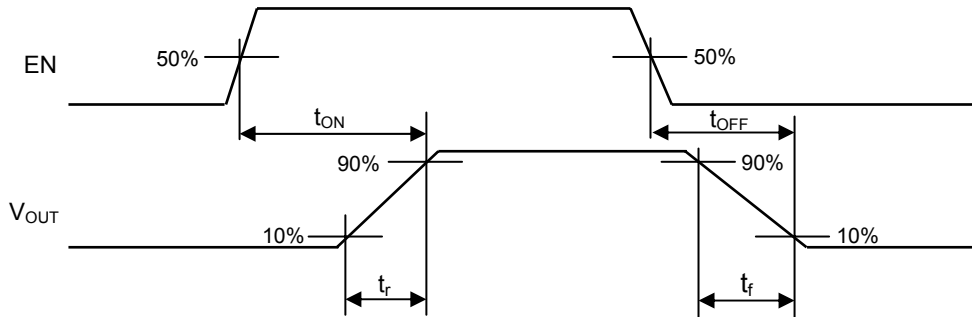
Figure 5. Timing Diagram
