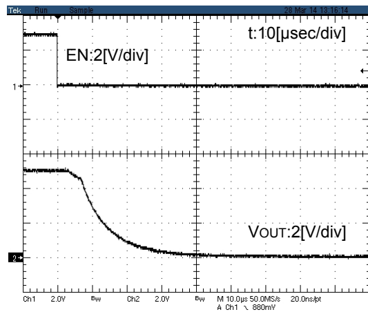
Figure.59 Turn off response 12 (BUS1DJC3GWZ VIN=5V)
