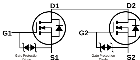
Internal Schematic
