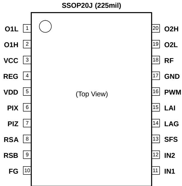
Figure 3. LV88561JA Pin Assignment
