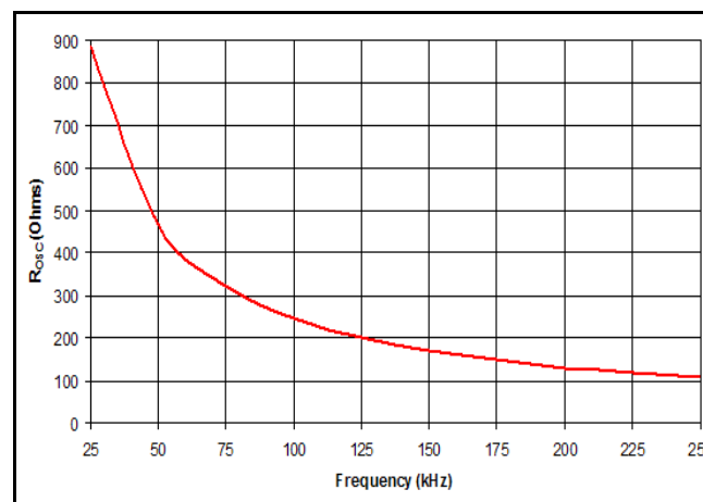
Figure 6: Oscillator Frequency vs. R_{OSC} Resistance
