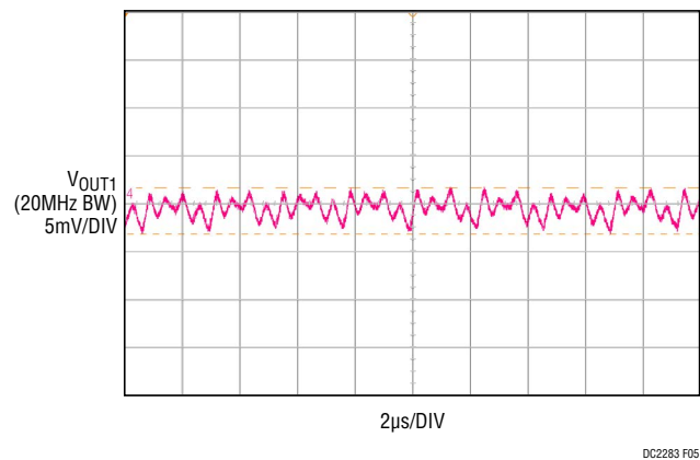
Figure 5. Output Voltage Ripple at V_{IN} = 12V , V_{OUT1} = 1V , I_{OUT} = 160A ( I_{OUT0} = 40A , I_{OUT1} = 120A )
