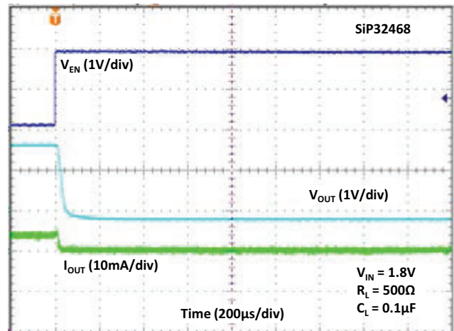
Fig. 33 - Turn-off Time
