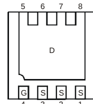
BOTTOM VIEW Pin Configuration
