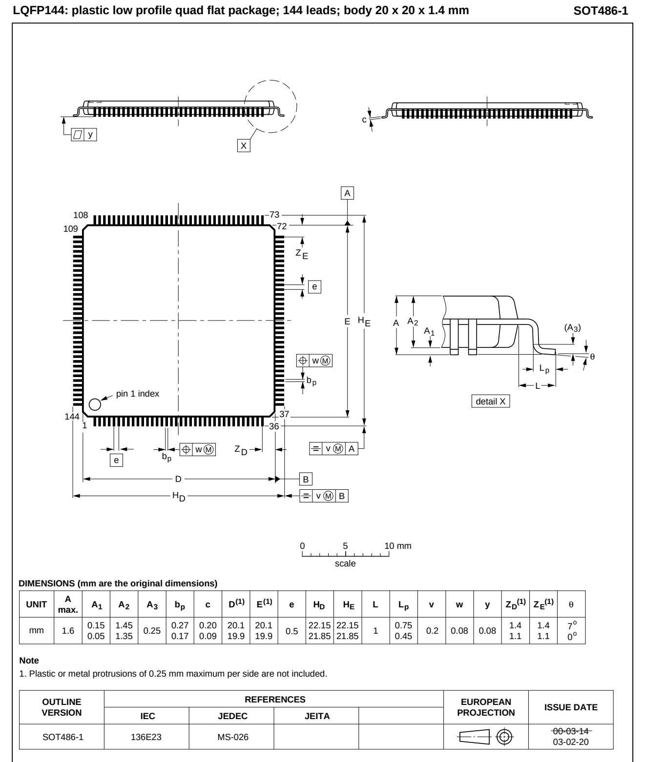
Fig 17. Package outline SOT486-1 (LQFP144)
