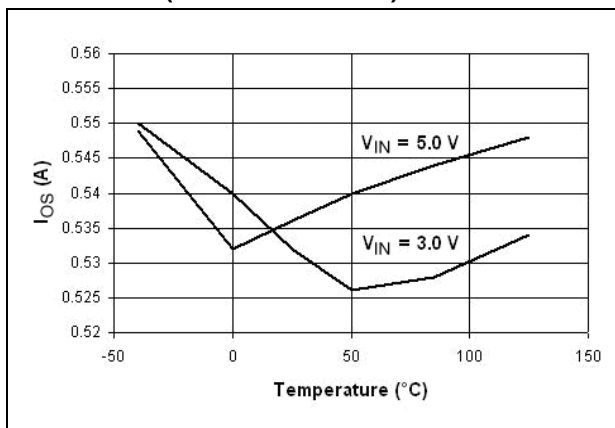
Figure 23. I_{OS} vs. temperature (STMPS2141/2151)
