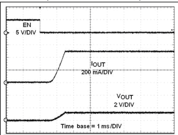
Figure 16. OC protection at V_{OUT} = 5.0\text{ V} (STMP2141/2151 - detail)
