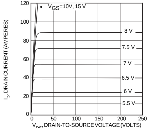
FIGURE 2, HIGH OUTPUT CHARACTERISTICS
