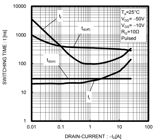
Fig.11 Switching Characteristics
