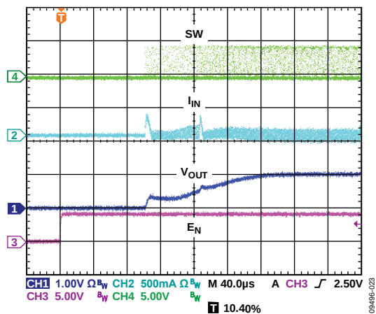
Figure 27. Startup, V_{OUT} = 0.8V , I_{OUT} = 10mA
