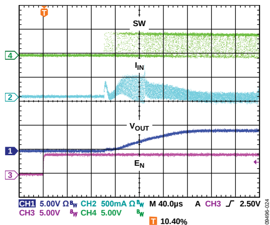
Figure 28. Startup, V_{OUT} = 3.3V , I_{OUT} = 10mA
