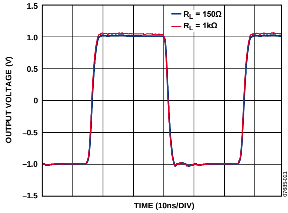
Figure 25. Large Signal Transient Response vs. Load Resistance
