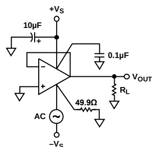
Figure 44. Negative Power Supply Rejection
