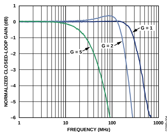
Figure 2. Frequency Response
