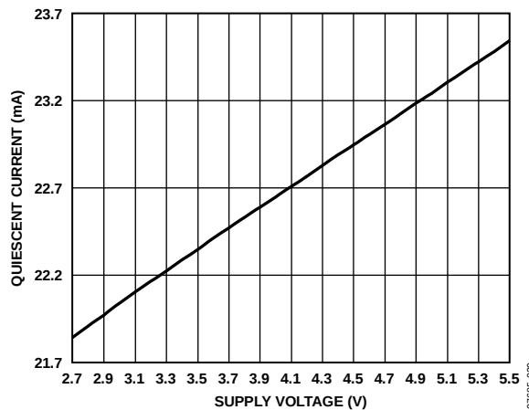
Figure 28. Quiescent Current vs. Supply Voltage
