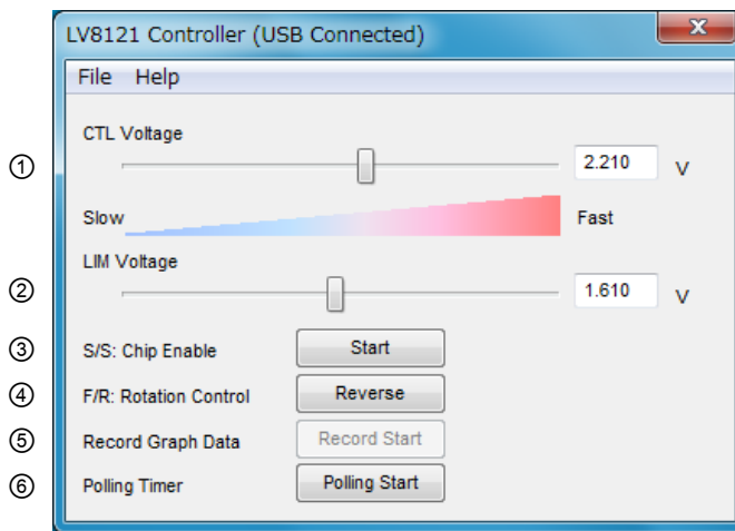
Figure 5. Controller window
