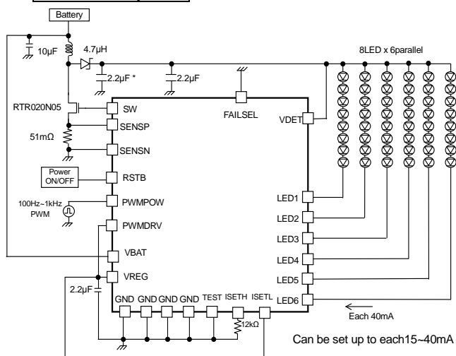
Figure 48. 8 seriesx 6 parallel, LED current 40mA setting Power control PWM application
