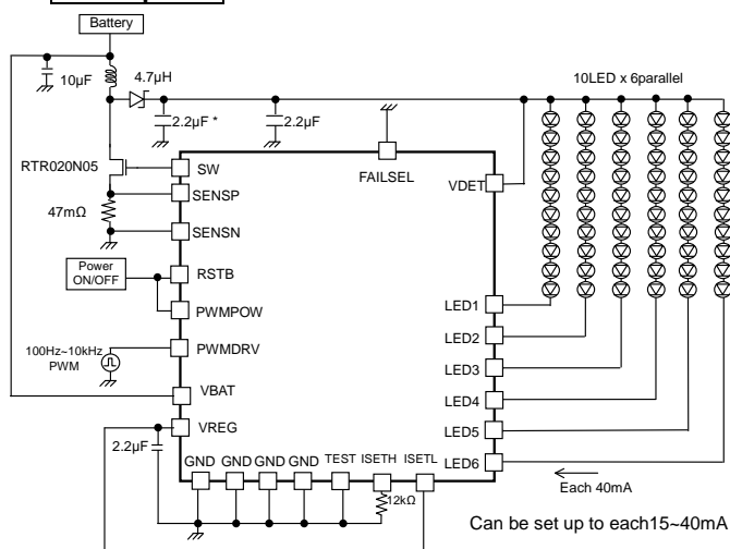
Figure 47. 10 seriesx6 parallel, LED current 40mA setting Current driver PWM application
