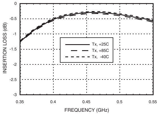
Insertion Loss vs. Temperature, Tx with 457 MHz Tuning
