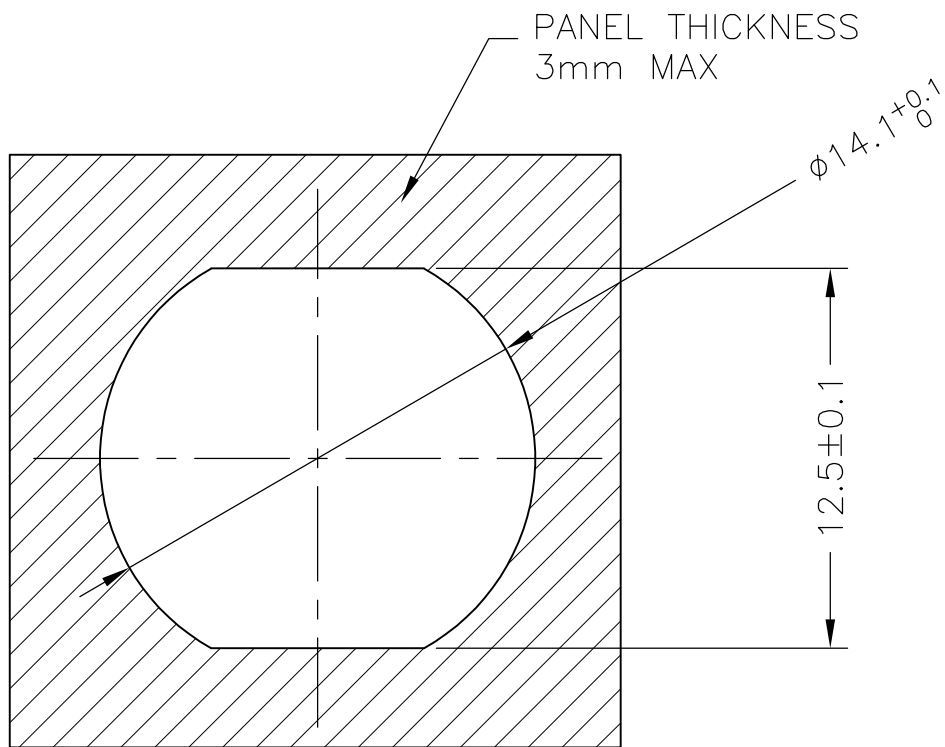
PANEL CUTOUT
