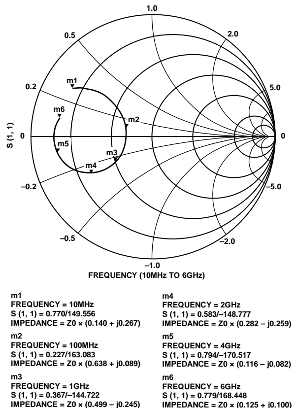
Figure 140. Simulated Smith Chart Showing the DAC Output Impedance, Z_o = 100 \Omega
