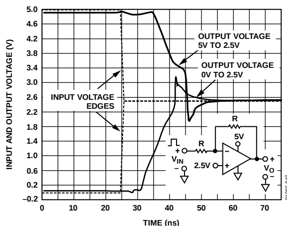
Figure 49. Overload Recovery, G = -1 , V_S = 5\text{ V}
