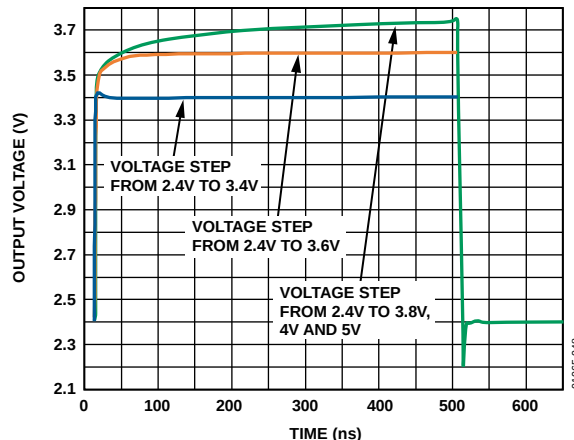
Figure 48. Pulse Response for G = 1 Follower, Input Step Overloading the Input Stage
