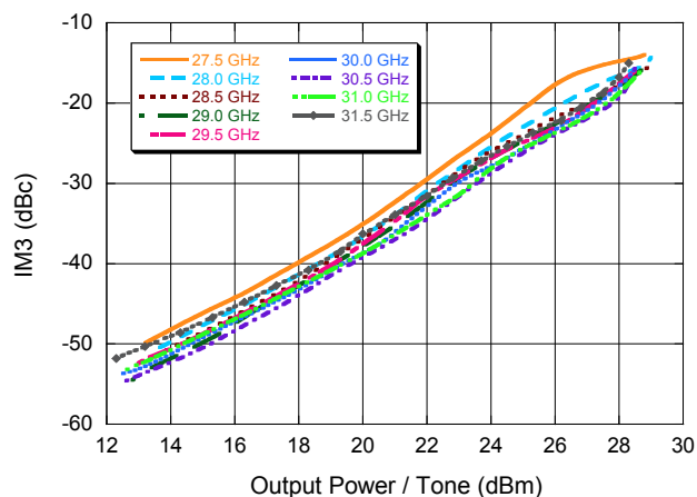
IM3 Level vs. P_{OUT} (dBm/toner)
