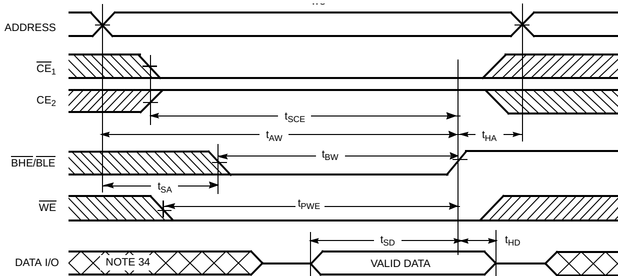
Figure 9. Write Cycle 4 ( \overline{\text{BHE/BLE}} Controlled, \overline{\text{OE}} LOW) [32]
