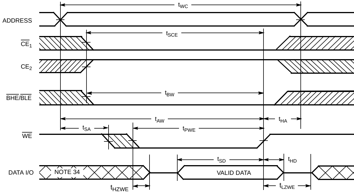
Figure 9. Write Cycle 4 ( \overline{\text{BHE/BLE}} Controlled, \overline{\text{OE}} LOW) [32]
