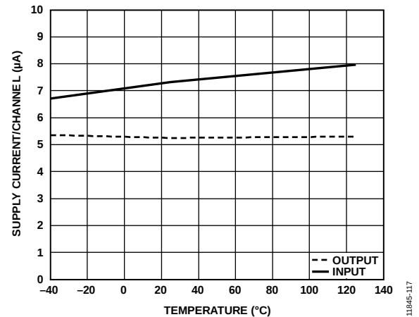
Figure 21. Typical Input and Output Supply Current per Channel vs. Temperature for V_{DDX} = 2.5 V, Data Rate = 100 kbps
