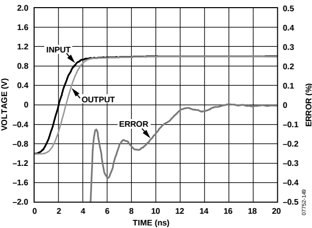
Figure 49. Settling Time
